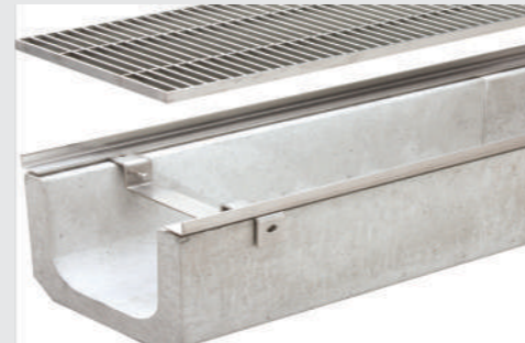
MĂNG & GRATING GUTTER & GRATING
